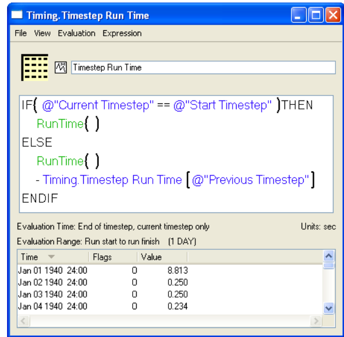
Figure 1: Expression Slots showing how the RunTime function can be used. Note, both are configured to evaluate at “End of Timestep, current timestep only”
