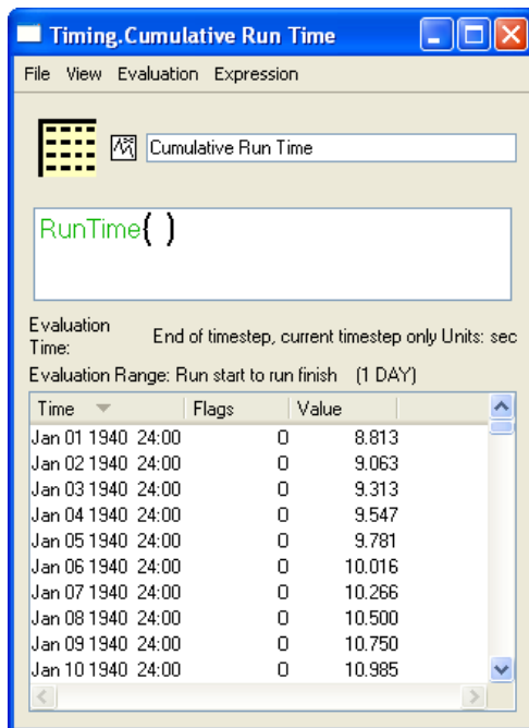
Figure 1: Expression Slots showing how the RunTime function can be used. Note, both are configured to evaluate at “End of Timestep, current timestep only”
